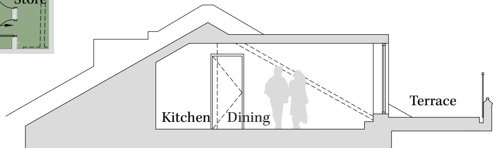
Section - First Floor NTS
