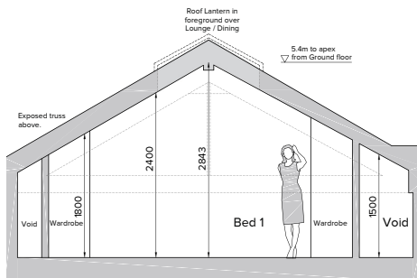
Section Through Mezzanine
